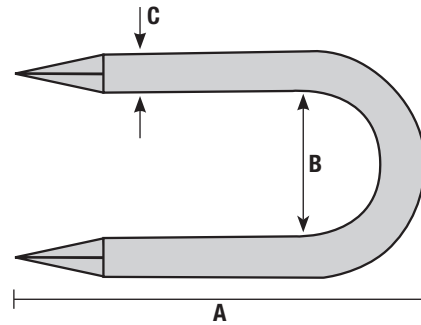
Diamond (Rolled) Point Staple
