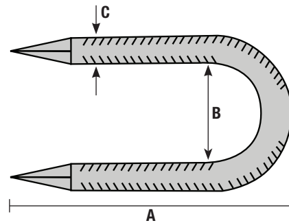
Serrated Diamond (Rolled) Point Staple
